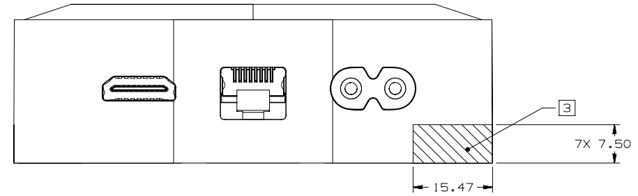
ANTENNA KEEPOUT
