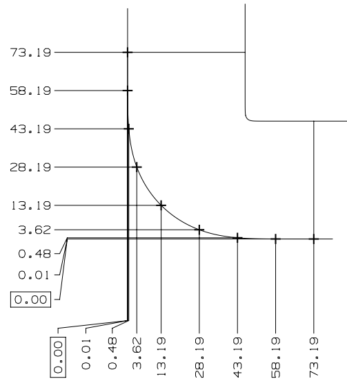
DETAIL A
