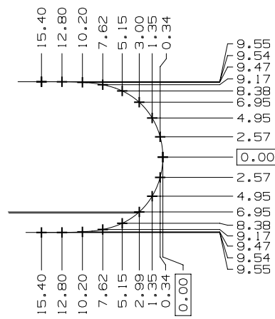
DETAIL C
