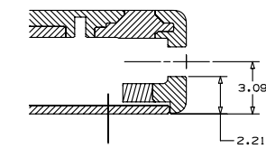
SECTION AB-AB SPEAKER HOLES
