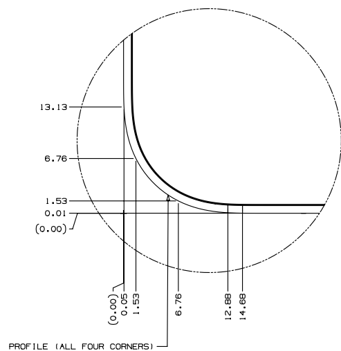
PROFILE (ALL FOUR CORNERS) DETAIL M
