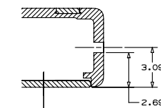
SECTION AA-AA SIDE MIC HOLE
