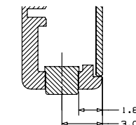
SECTION Y-Y VOLUME BUTTONS
