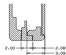
SECTION W-W SIM TRAY (CELLULAR ONLY)
