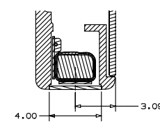
SECTION X-X INDUCTIVE CHARGING WINDOW FOR PENCIL
