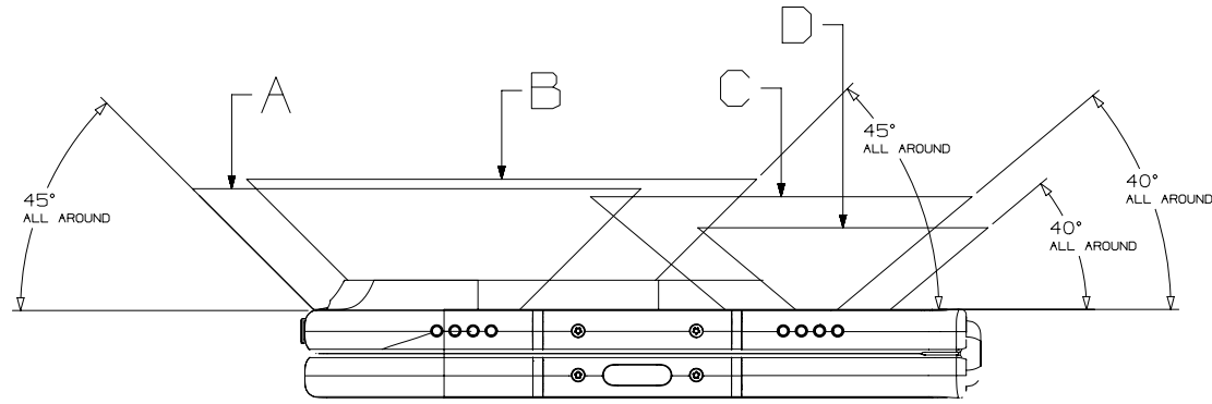
MAGSAFE AND TAPTIC ENGINE KEEP OUT ZONES
