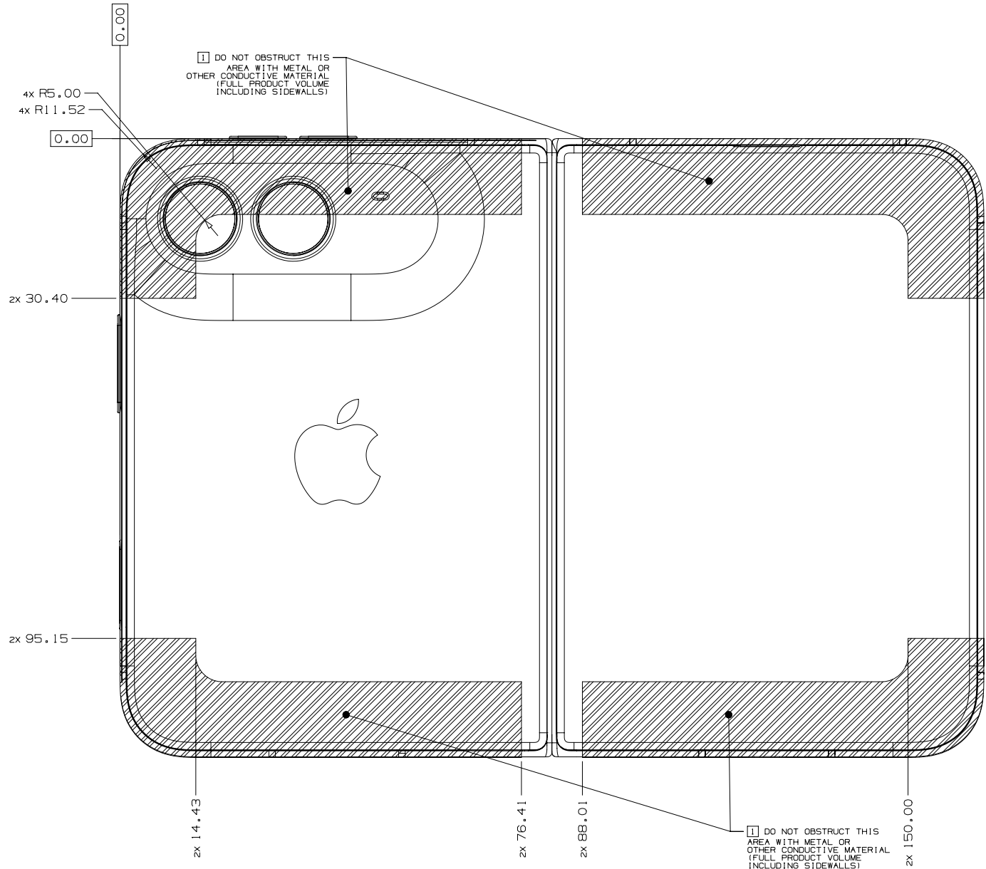
BAND ANTENNA KEEP OUT ZONES
