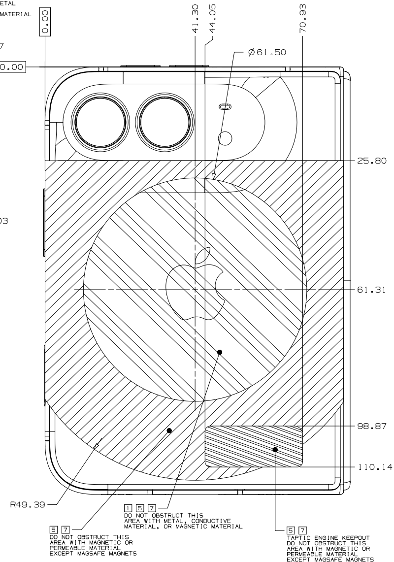
MAGSAFE AND TAPTIC ENGINE KEEP OUT ZONES
