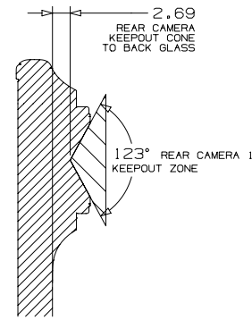
SECTION S - S
