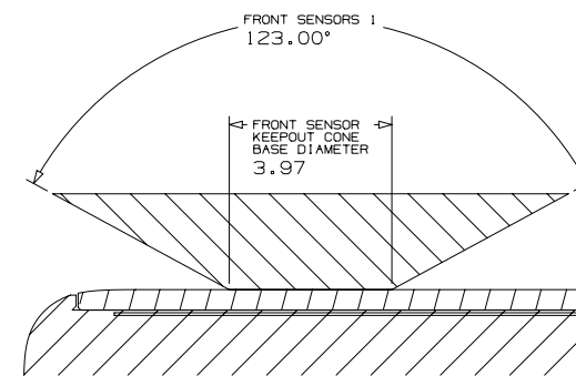
SECTION U - U
