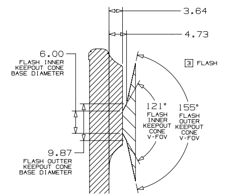
SECTION T - T
