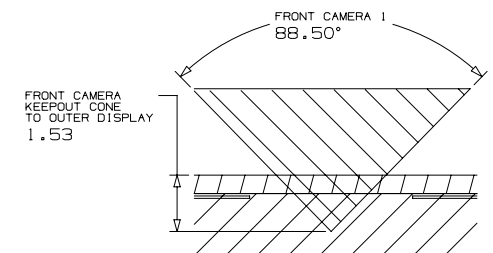
SECTION P - P
