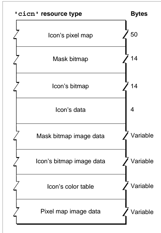
Figure 4-18 Format of a compiled color icon ('icn') resource
